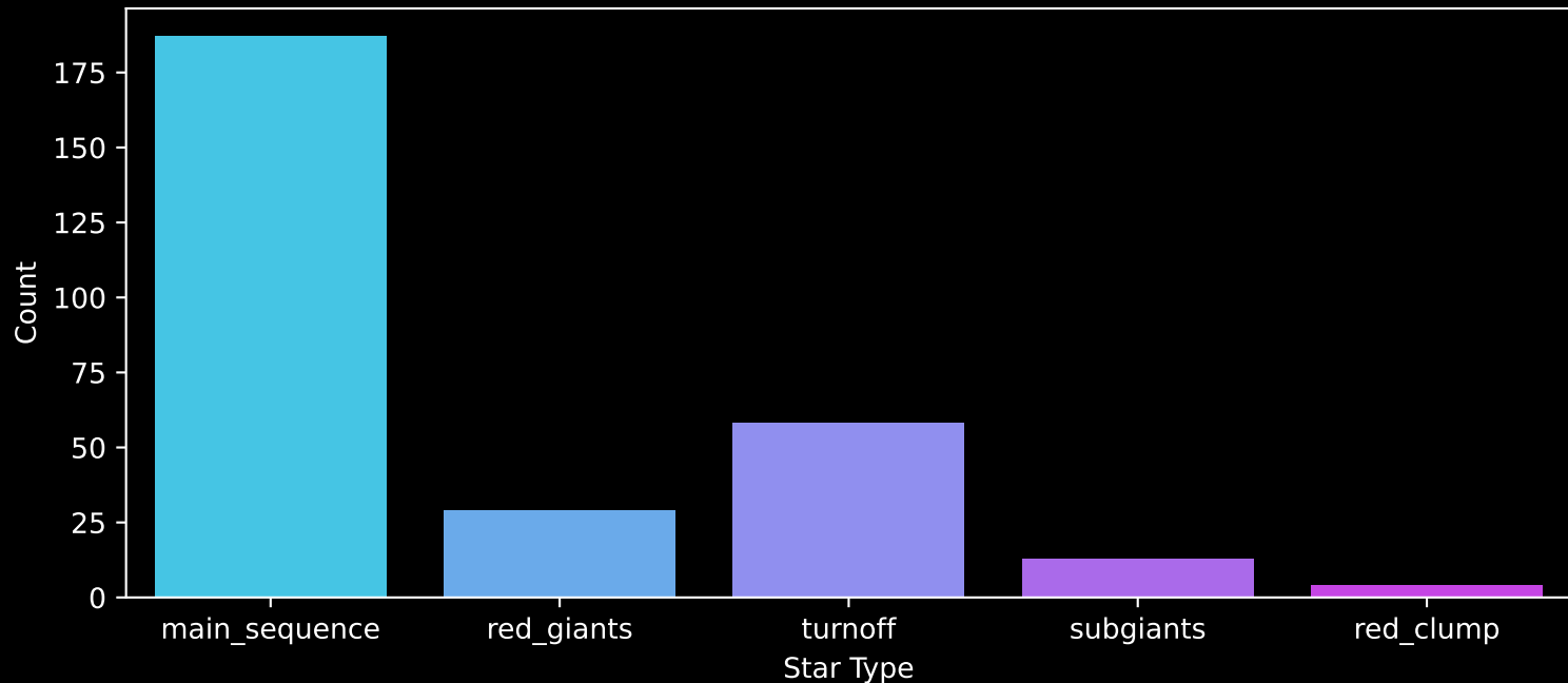
GALAH DR4 Field: [6860] Count plot of Star Type
