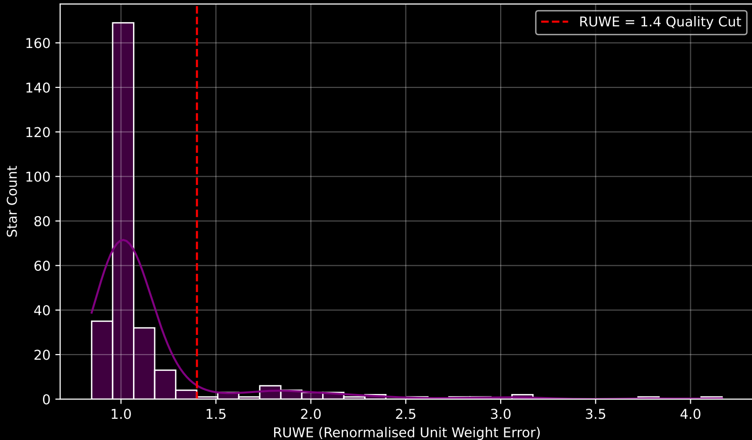
GALAH DR4 Field [6860] RUWE Distribution (n= 284)
