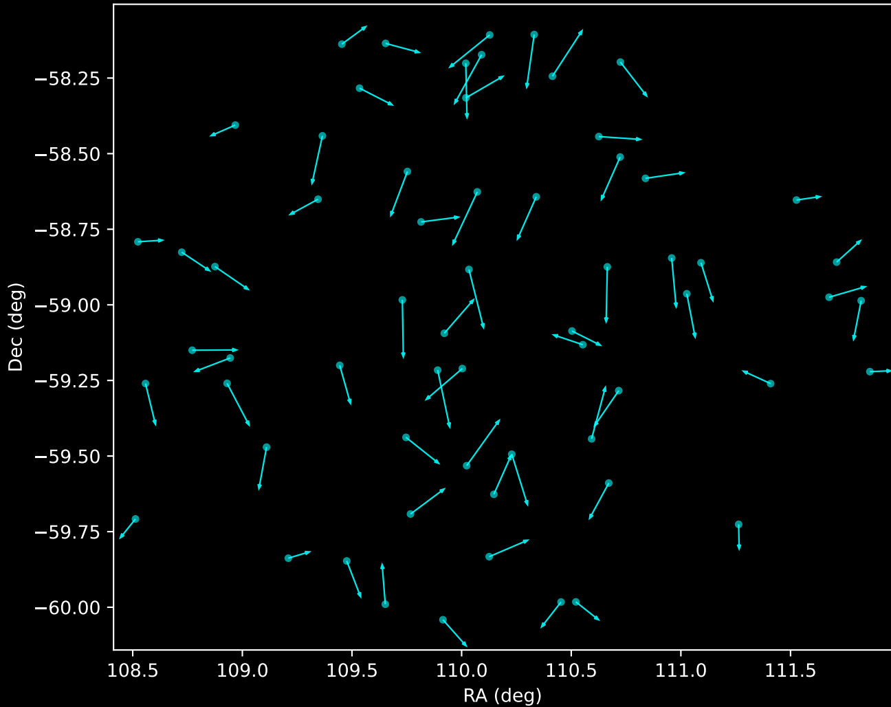
GALAH DR4 Noise Stream Proper Motion Vectors (n=63)
