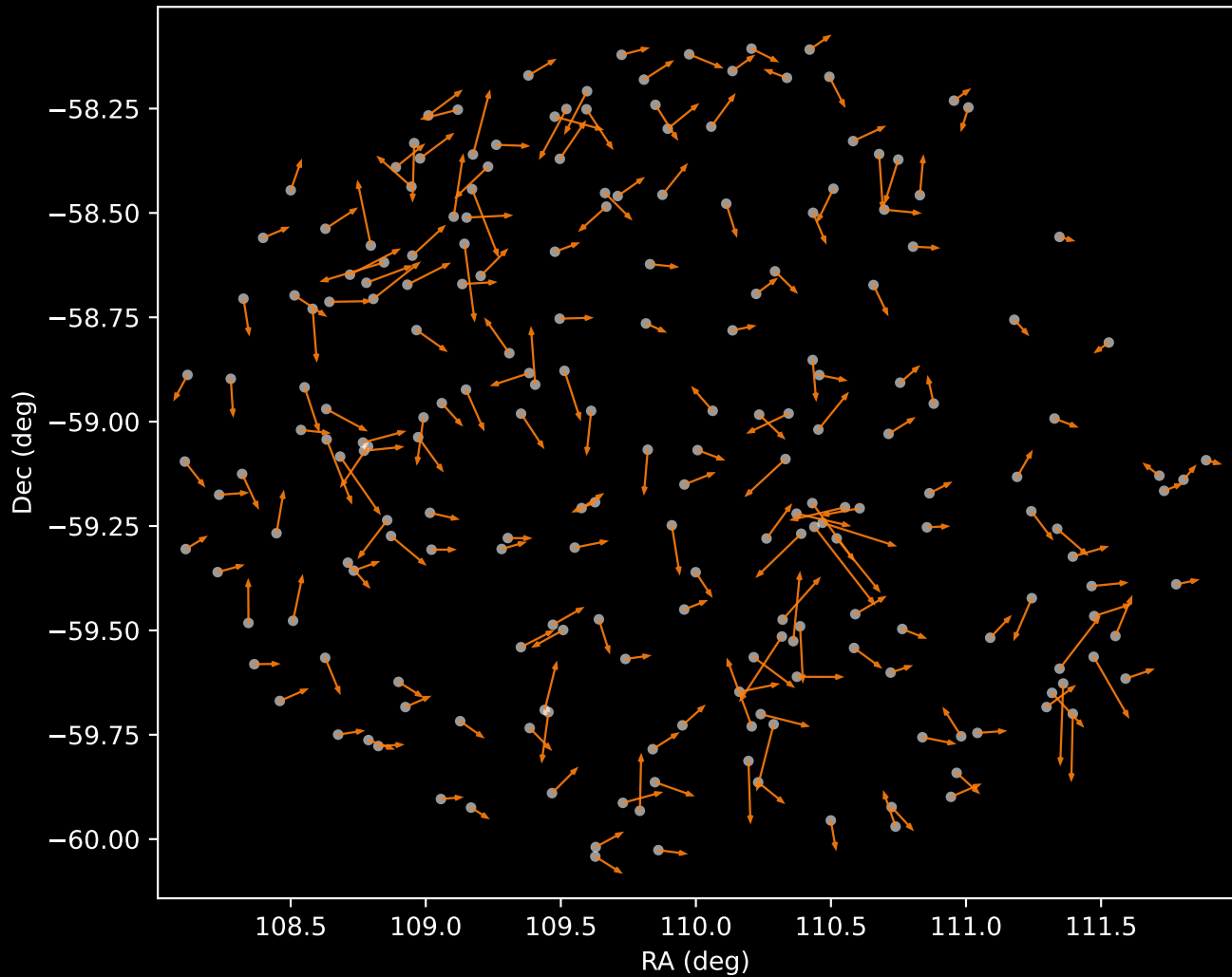
GALAH DR4 Cluster 2 Proper Motion Vectors (n=213)
